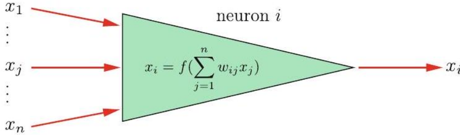
Figure 10.1: The structure of a formal neuron, which applies the activation function f to the weighted sum of all inputs
